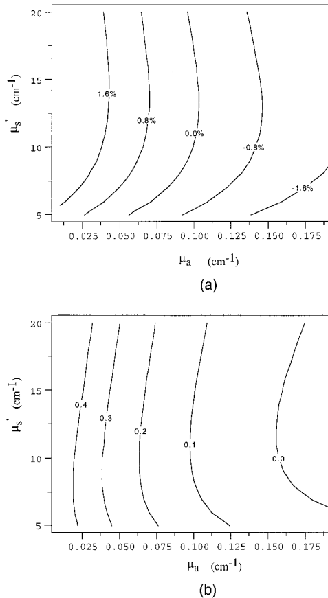
Fig. 6. Effect of Fresnel reflections on measured ac and phase. The index of refraction mismatch between background and cylinder media is n_{\text{background}} = 1.33 versus n_{\text{object}} = 1.45 . The infinite cylinder is centered between the source and the detector, which are separated by 5.0 cm. The background medium absorption and the scattering coefficients are \mu_a = 0.1 \text{ cm}^{-1} and \mu_s' = 10 \text{ cm}^{-1} , whereas the absorption and the scattering coefficients of the cylinder vary ( 0.01 \text{ cm}^{-1} < \mu_a < 0.2 \text{ cm}^{-1} , 5 \text{ cm}^{-1} < \mu_s' < 20 \text{ cm}^{-1} ). (a) Perturbation in measured ac intensity due to Fresnel reflections. As the cylinder becomes more (less) transparent than the background medium, the measured ac intensity is increased (decreased) owing to Fresnel reflections. (b) Difference in measured phase caused by Fresnel boundary conditions. This phase lag increases as the absorption coefficient of the cylinder decreases, reaching a maximum value of 0.5^\circ when \mu_a = 0.01 \text{ cm}^{-1} .
