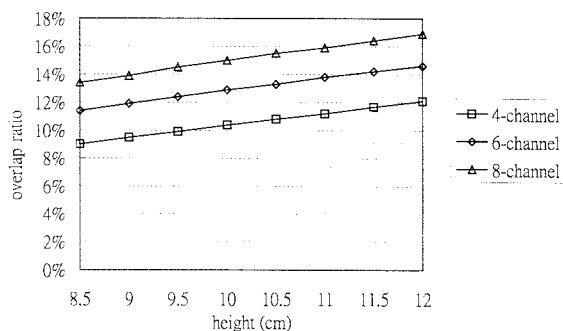
Fig. 15. Optimal volume overlap ratio for the 12-cm-radius head phased array at different height and different number of ports.
