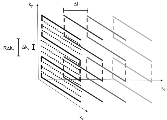
FIG. 2. The k_x - k_y - t -space trajectory for single-shot spatial-spectral encoding. Phase-encoding lines are measured with k_y -spacing R\Delta k , where R(= 4) denotes the acceleration factor. Target k_y -spacing after SENSE reconstruction is \Delta k . Each readout module, which consists of four forward and four reverse k_x - k_y -space-encoding segments, is traversed forward and backward, and repeated N -times with spacing \Delta t to encode N spectral points. Data are only collected during the horizontal segments of the trajectory ( 69 \times 50 mm; 300 \times 300 DPI).
