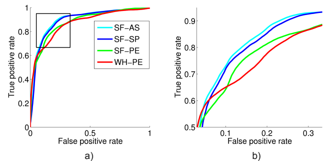
Figure 7: Receiver operating characteristic (ROC) curves for the competing methods. (a) Complete curve. (b) Detail of the top left corner (the “elbow”) of the curve, which is where the operating point would typically be located. This region is marked with a box in (a).
