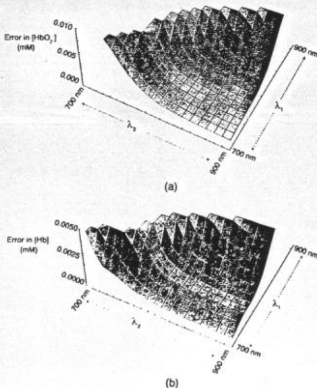
Fig. 1 Errors in (a) [\text{HbO}_2] and (b) [\text{Hb}] as a function of the two wavelengths employed ( \lambda_1, \lambda_2 ). The values of the standard errors in \mu_a^{\lambda_1} and \mu_a^{\lambda_2} have been set equal to 0.001 \text{ cm}^{-1} .
