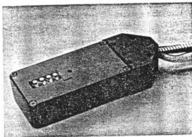
Fig. 5 Photograph of a prototype of the measuring head of the frequency-domain tissue spectrometer built by ISS, Inc. (Champaign, Illinois).
