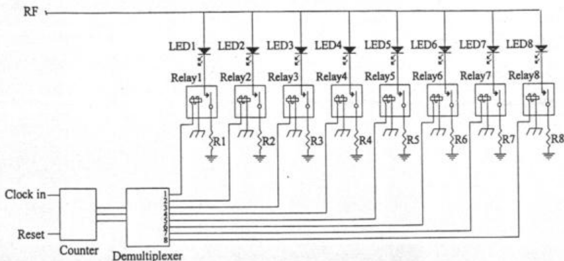
Fig. 3 Schematic diagram of the measuring head circuit. The inputs are the radio-frequency oscillating signal (from a frequency synthesizer), a clock signal, and a reset pulse (both from the computer). The counter (RCA CD4024) counts the waves of the clock signal and continuously transmits the number (mod 8) to the demultiplexer (74HCT238). The enabled line of the demultiplexer, which closes the corresponding relay (Magnecraft W171 DIP-2), is then changed at the frequency of the clock. The reset pulse is sent at the beginning of the measurement to start the sequence always with the same LED.
