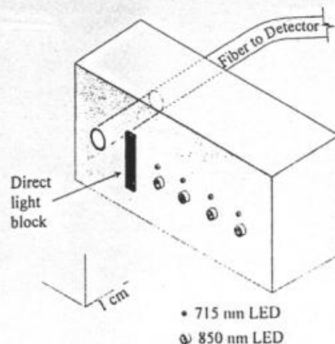
Fig. 2 Design of the measuring head of the tissue spectrometer. In a measurement, the shaded surface, on which the eight LEDs and the tip of the detector optical fiber are located, is placed in contact with the sampled medium. The light shield between sources and detector is used to block the light reflected at the surface of the medium.
