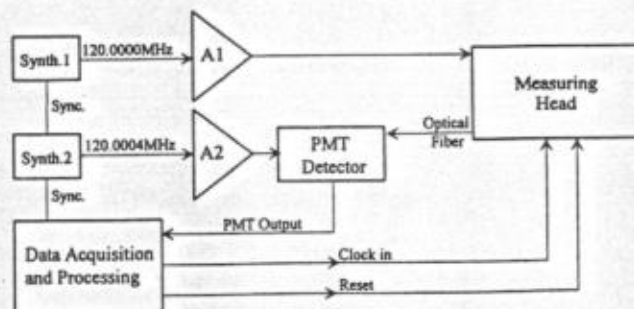
Fig. 4 Block diagram of the frequency-domain tissue spectrometer.
