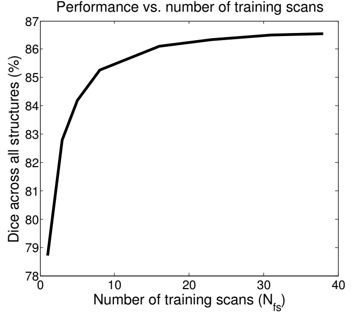
Figure 8: Mean Dice score (in %) for the FreeSurfer dataset as a function of the number of training scans of the FreeSurfer dataset N_{fs} . The pool of training scans also includes atlases from the other three datasets, such that the ratio of scans from the different datasets is approximately constant (see Table 4). The Dice scores are averaged over all structures and ten random selections of scans (except for N_{fs} = 1 , where we used all 38 left-out scans, and N_{fs} = 38 , where there is only one possible combination of atlases).
