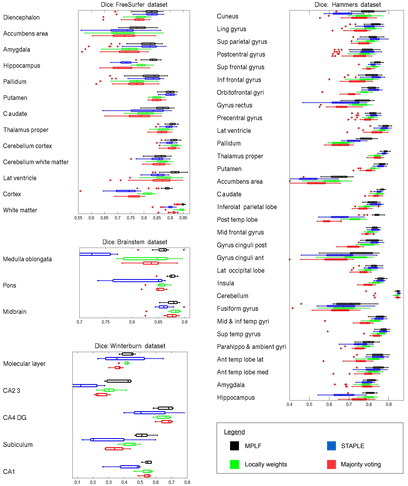
Figure 9: Box plots for the Dice scores corresponding to the four datasets. The central mark is the median, the box spans from the first to the third quartile, and the whiskers span the extreme data points not considered outliers (which are marked with red crosses).
