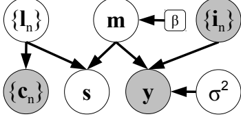
Figure 2: Graphical model for generalized semi-locally weighted voting. Shaded variables are observed.
