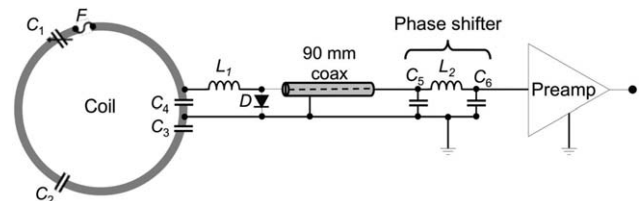
FIG. 3. Circuit schematic for coil elements with a long coaxial cable that allows placement of the preamplifier outside the PET FOV. To maintain a \lambda/2 phase shift, a pi phase shifter is located before the preamplifier chain.
