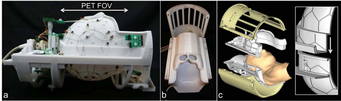
FIG. 2. The 31-channel PET/MR array coil is divided into an anterior and posterior part, with 15 and 16 channels, respectively. a: Side view of the array, with overlapping loop design and preamplifiers outside the FOV of the PET camera. b: Fit of the receive coil with cover into the local transmit coil. c: CAD design of the coil with an anterior and posterior part and a magnification of the mechanical rim system that allows for an overlapped loop design between the two coil parts.
