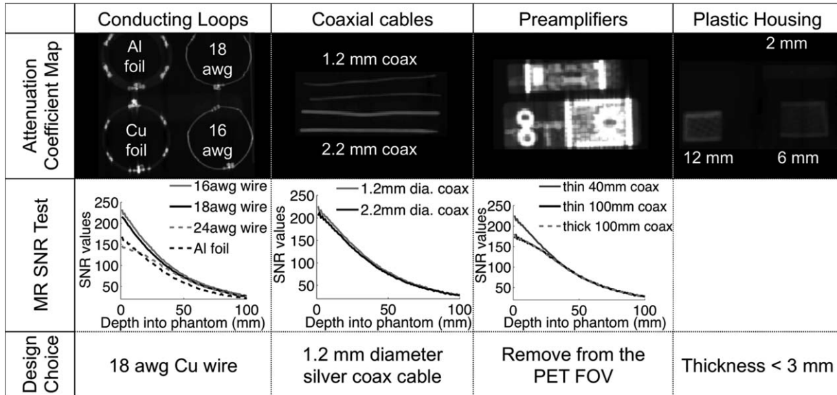
FIG. 1. 511 keV attenuation map of the main coil components that were evaluated for the design of the 31-channel PET/MR array coil (1st row), showing high attenuation of the preamplifiers and thick metal or plastic components. Each electrical component was tested for its MR SNR in a single-loop configuration on a water phantom (2nd row). The final design choices reflect the goal to reduce attenuation but preserve SNR for MRI (3rd row).
