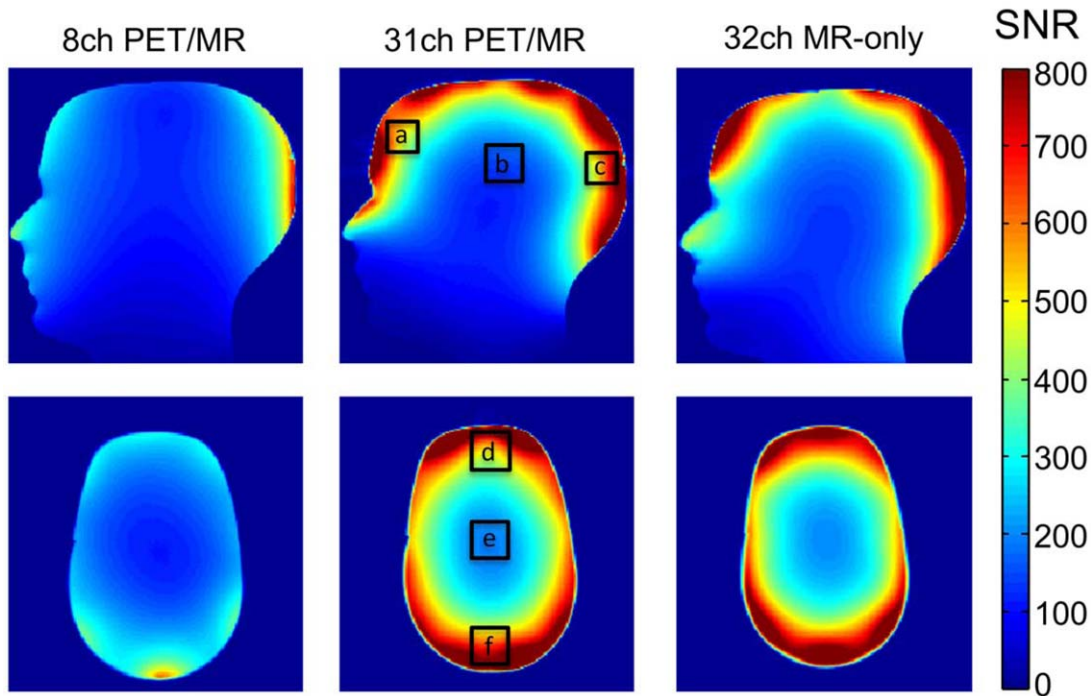
FIG. 5. Signal to noise maps of a human head-shaped water phantom (sagittal and axial slice) for the 8-channel PET/MR, the 31-channel PET/MR, and a standard 32-channel MR-only array. The gain in SNR compared with the 8ch PET/MR coil for the ROIs shown is: 2.3 (a), 1.6 (b), 1.7 (c), 2.2 (d), 1.8 (e), 2.1 (f). The SNR of the 31-channel PET/MR coil shows a large improvement compared with the 8-channel coil, and shows no overall SNR loss compared with the 32-channel MR-only array.
