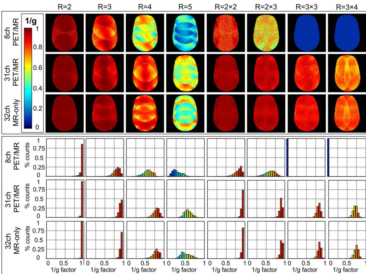
FIG. 6. Top: 1/g factor maps for the 8-channel PET/MR, the 31-channel PET/MR and the 32-channel MR-only array for acceleration factors R in 1D and 2D. Bottom: Corresponding histograms of 1/g factor maps for the three coils in comparison. Compared with the 8-channel PET/MR coil, the 31-channel PET/MR coil shows much higher 1/g factors values at all acceleration stages. Despite the design constraints for PET compatibility, the 31-channel PET-optimized array performs similarly to an MR-only array with an equivalent number of channels.
