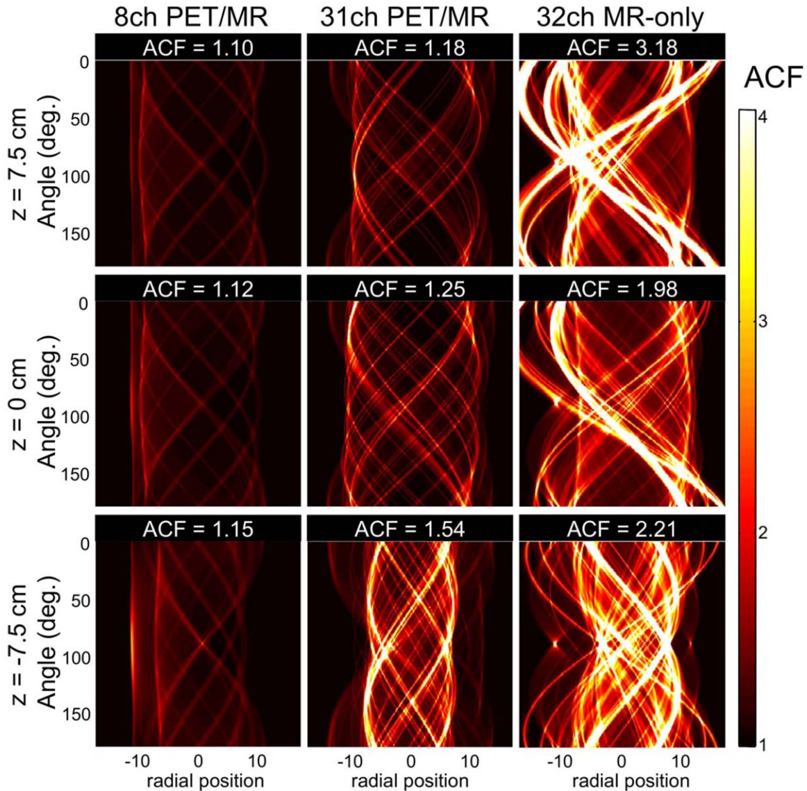
FIG. 8. Sinograms calculated from a forward projection of the CT scans (shown in Fig. 7) for z-positions -7.5 cm, 0 cm, and 7.5 cm. The mean attenuation correction factors (ACF) of the 31-channel PET/MR coil, the 8-channel PET/MR, and a standard MR-only 32-channel coil are shown for each slice. This estimation shows that while the 31-channel PET/MR coil would only attenuate between 18 to 54% of the 511 keV photons (similar to the 8-channel PET/MR coil), an MR-only standard 32-channel coil would attenuate much more photons (up to 218%).
