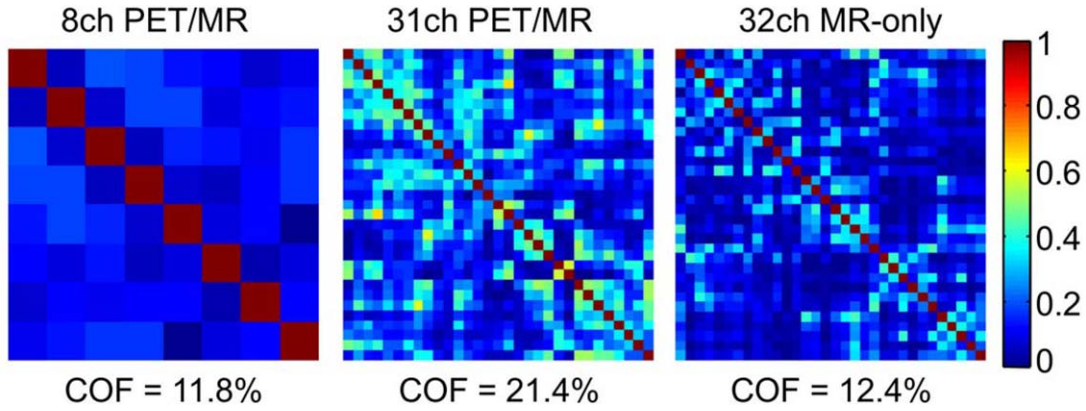
FIG. 4. Noise correlation matrices for the 8-channel PET/MR, the 31-channel PET/MR, and the 32-channel MR-only array. The average noise correlation is 11.8%, 21.4%, and 12.4%, respectively.
